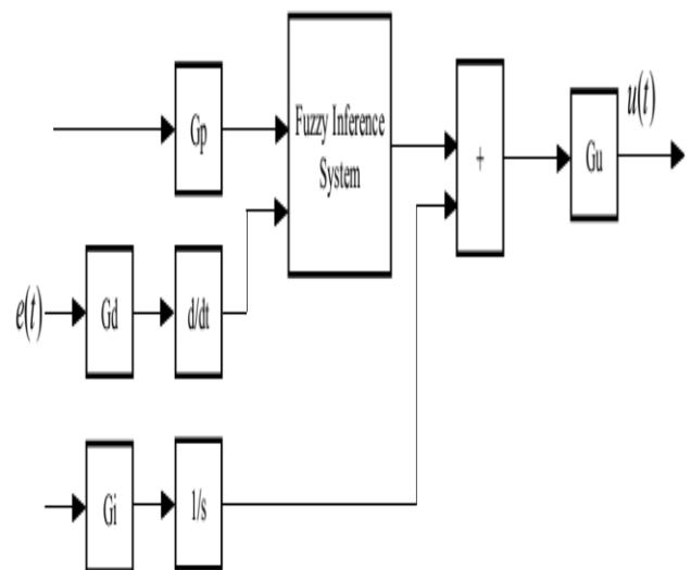
Fig.11. Structure of hybrid fuzzy controller
