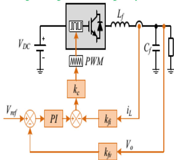
Fig.2. Control method of output voltage
