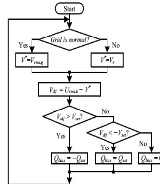
Fig.7. Control method of amplitude tracking
