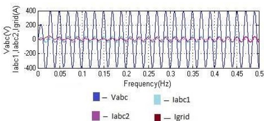
Fig.21. Simulation waveform of GTM with Fuzzy logic controller
