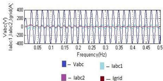
Fig.19. Simulation results for mode transfer from GTM to ILM: Phase voltages (Vabc), Phase currents (Iabc1, Iabc2) and Grid current (Igrid)
