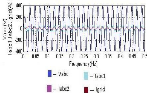
Fig.13. Simulation results for GTM:Phase voltages (Vabc), Phase currents (Iabc1, Iabc2) and Grid current (Igrid)
