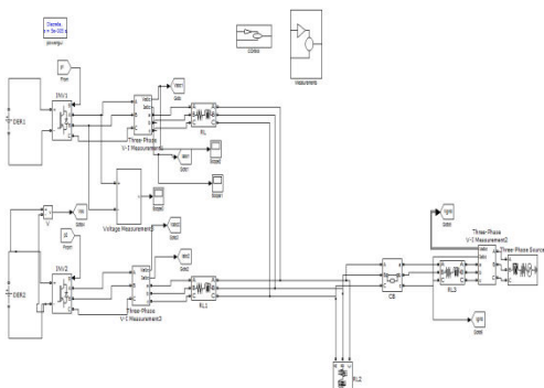
Fig.18. Matlab and Simulink circuit for mode transfer from GTM to ILM
