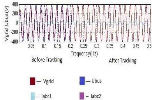
Fig.15. Simulation results for grid-tracking in ILM : Phase voltages (Vabc), Phase currents (Iabc1, Iabc2) and Grid current (Igrid)
