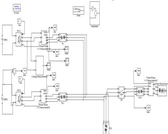
Fig.14. Matlab and Simulink circuit for grid-tracking in ILM
