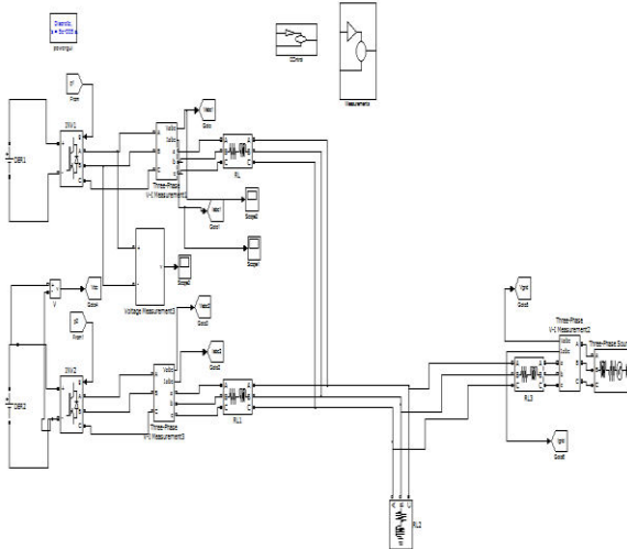
Fig.12. Matlab and Simulink Circuit diagram for GTM
