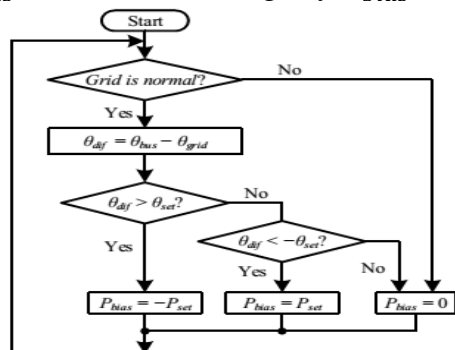
Fig.6. Control method of phase tracking
