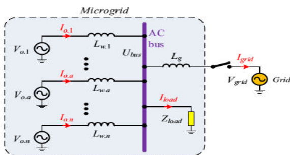
Fig.1. Diagram of microgrid system
