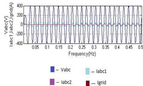
Fig.17. Simulation results for mode transfer from ILM to GTM: Phase voltages (Vabc), Phase currents (Iabc1, Iabc2) and Grid current (Igrid)
