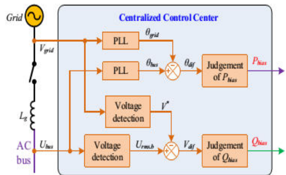
Fig.5. Grid-tracking control strategy
