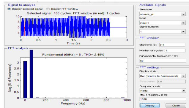
Fig 17 FFT analysis of THD with PI controller
