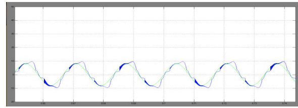
Fig 15 Simulation results of the proposed system: grid current ( i_g ) and load current ( i_l ) with fuzzy logic controller
