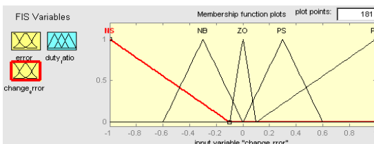
Fig. 7. The Membership Function plots of change error
