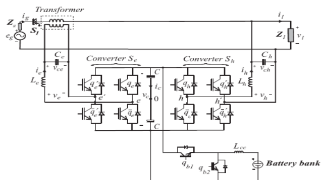
Fig.1 (b) Single-phase universal active filter conventional topology with UPS features.
