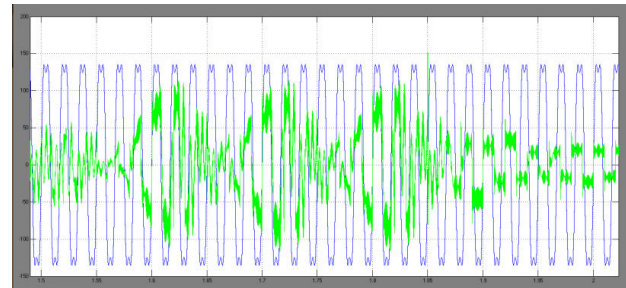
Fig 16 Simulation results of the proposed system: grid voltage ( e_g ) and load voltage ( v_l ) with fuzzy logic controller
