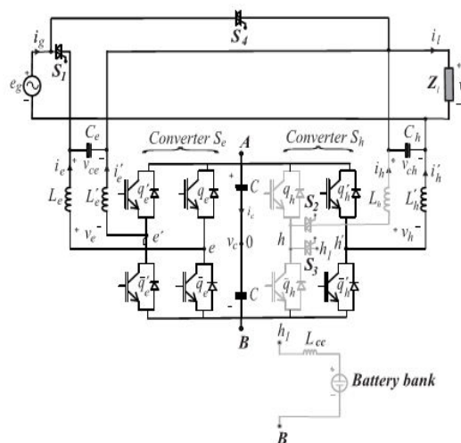
Fig.2 (b) three-leg mode
