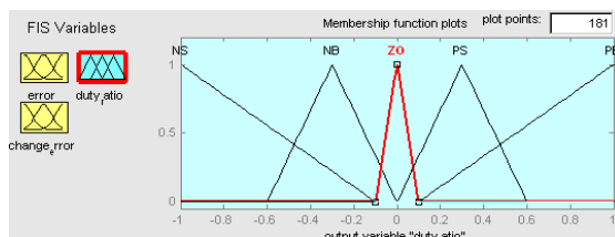
Fig. 8. the Membership Function plots of duty ratio
