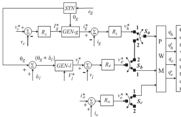
Fig.3. Control block diagram of the proposed configuration
