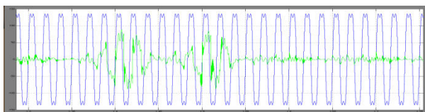
Fig 12 Simulation results of the proposed system: grid voltage ( e_g ) and load voltage ( v_l ).
