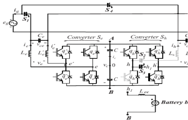
Fig.2 (c) three-leg mode charging the battery bank
