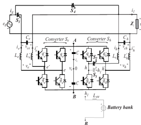
Fig.2 (a) four-leg mode
