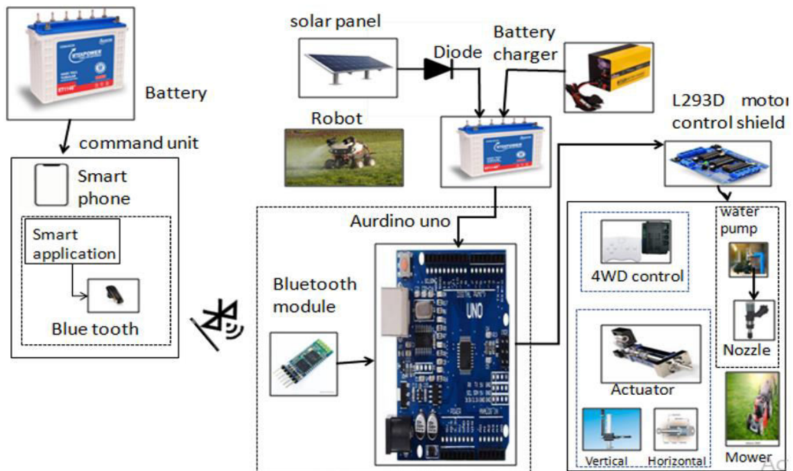
Figure 2: Block diagram of proposed system
