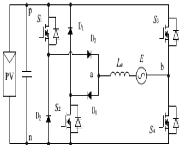
Fig.4. Proposed dual buck full bridge inverters with single inductor.
