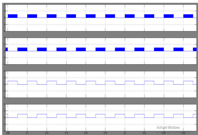
Fig 5: The simulated switching signals or pulses of the dual buck inverters.
