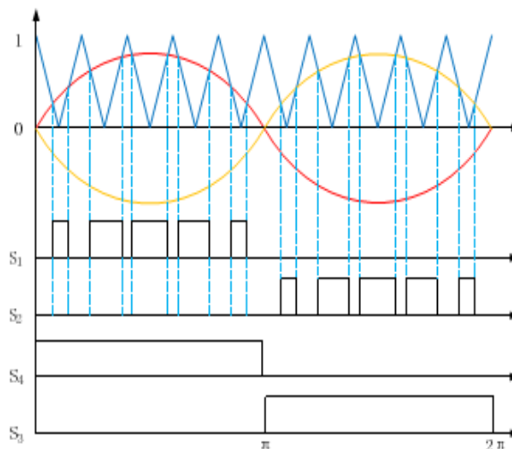
Fig.6. The switching signals of the proposed inverters.
