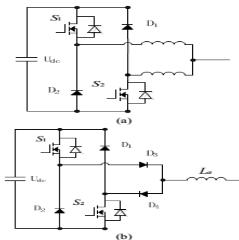
Fig.3. (a) Traditional dual buck phase leg (b) proposed dual buck phase legs with series connected diodes and single inductor.
