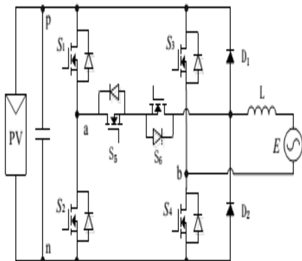
Fig.2. Traditional Dual buck full bridge inverter with single inductor.
