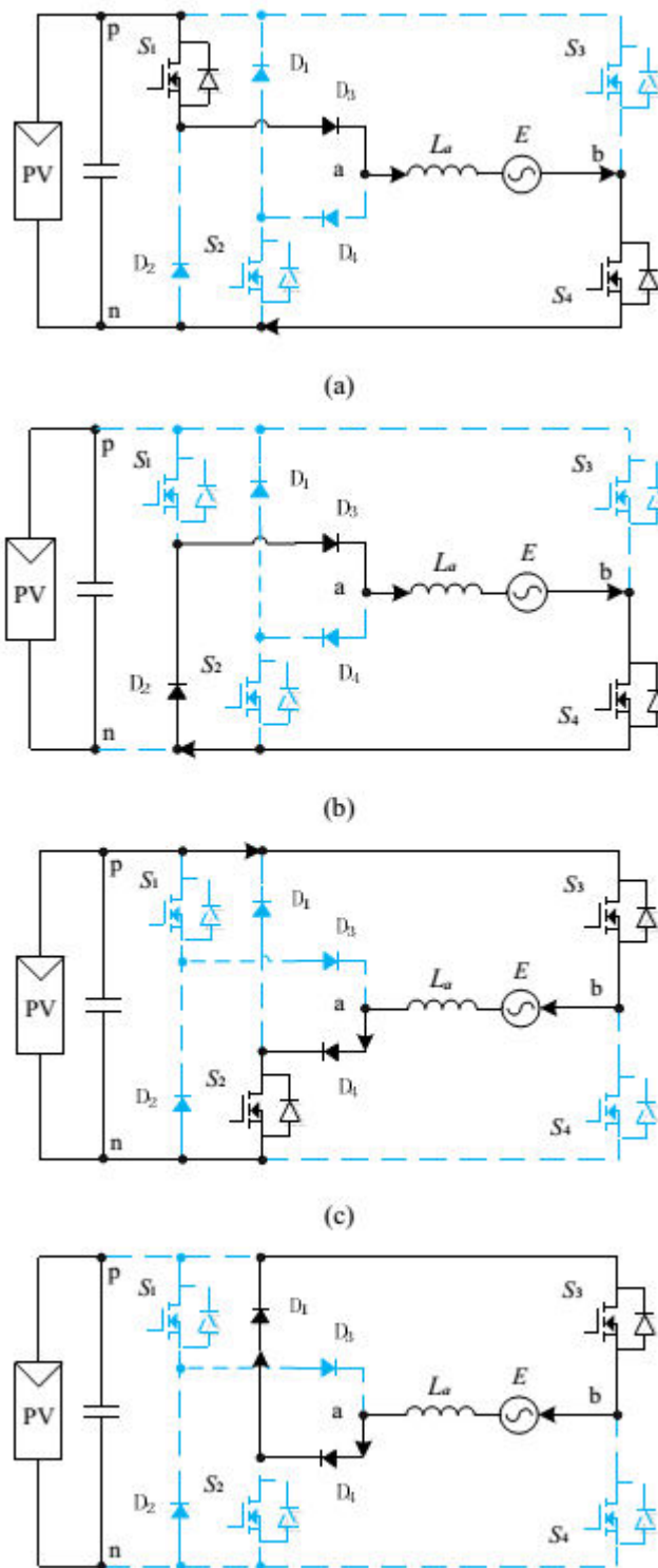
Fig.5. Four working modes of the proposed dual buck full bridge inverter with single inductor in Fig.3.4.
