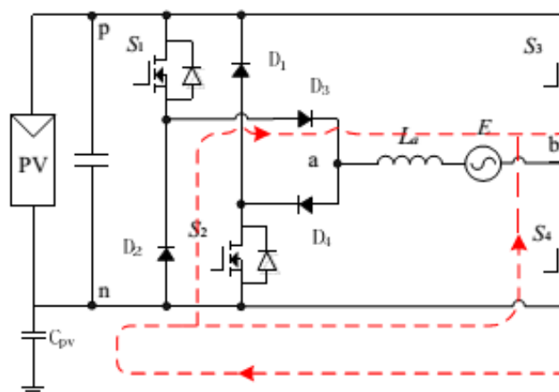
Fig.7. the equivalent common-mode circuit of the proposed single inductor dual buck inverter.
