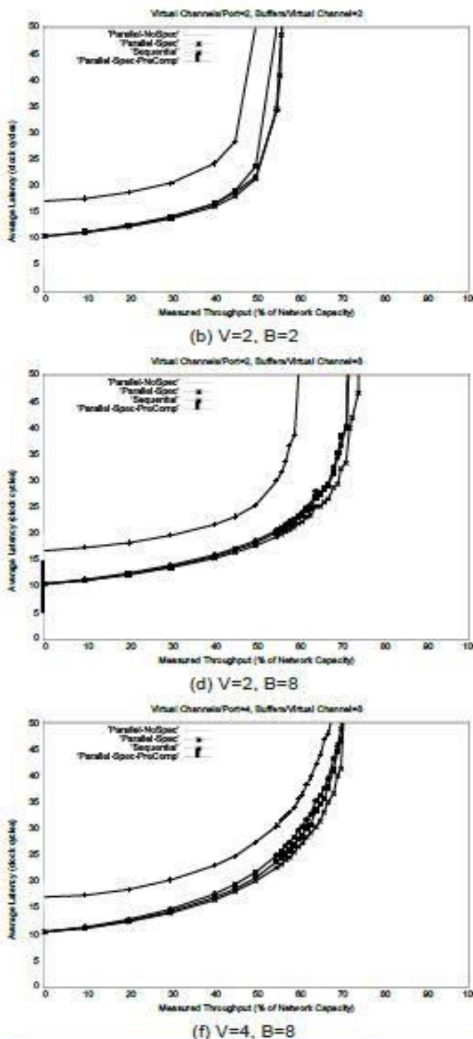
Figure 9. Latency versus throughput for a number of different VC and switch allocation implementations (5-flit packets). For each graph, V is the number of virtual-channels per input port and B is the number of buffers per virtual-channel.
