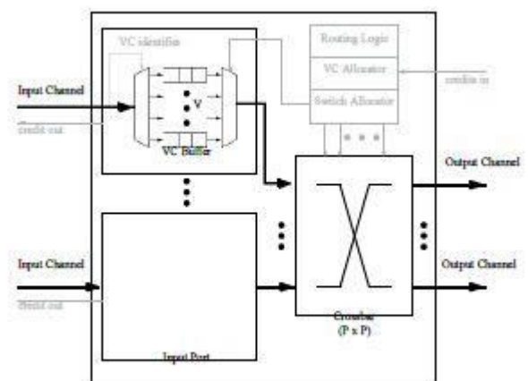
Figure 2. Virtual-Channel Router
