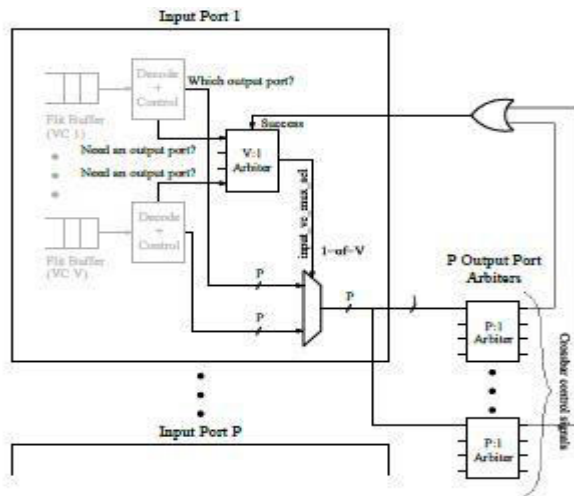
Figure 4. Switch Allocation Logic
