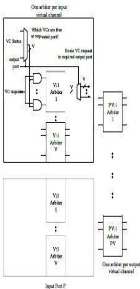
Figure 3. Arbitration complexity of a virtual channel allocator. In this example, the routing
