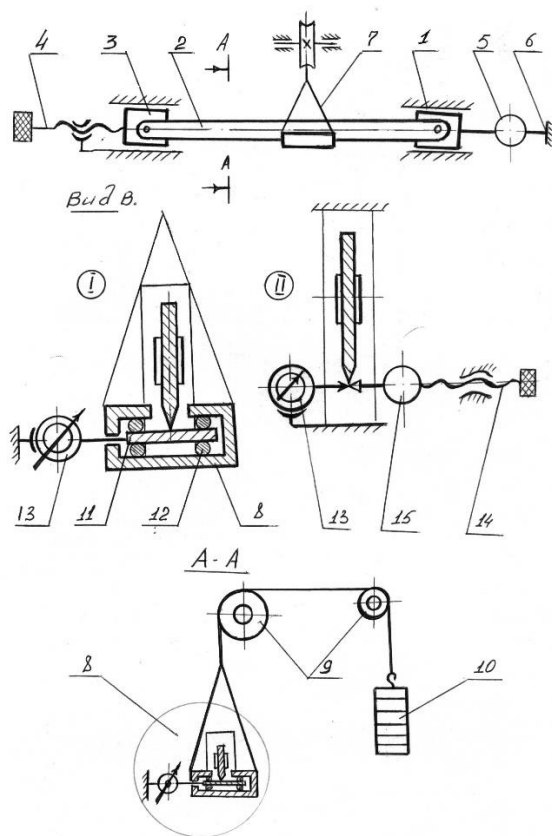
Fig. 1. Schematic diagram of the experimental installation
