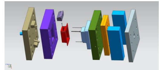
Exploded view
