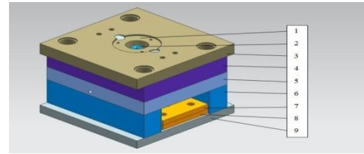
Mould construction
