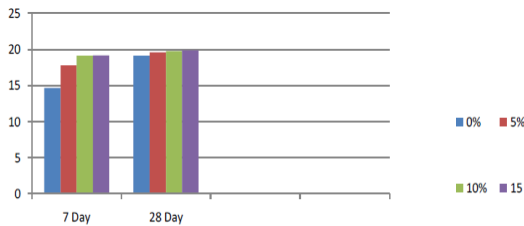
Fig. (b) Compressive Strength for M20 Grade Concrete
