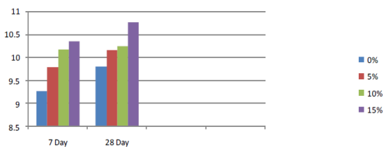
Fig.4.2. Strength Results.
