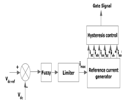
Fig.9. Conventional fuzzy controller
