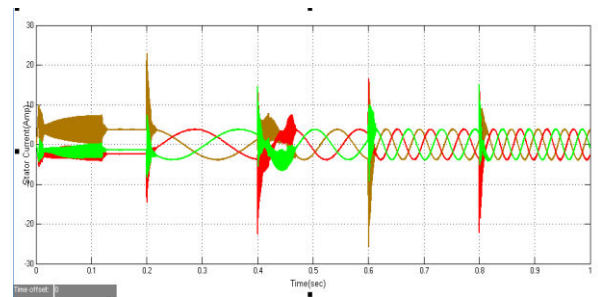
(b) PMSM Iabc Stator current
