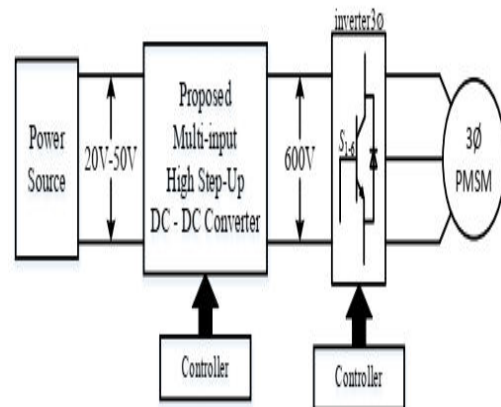
Figure 4. The multi-input converter for PMSM drive system
