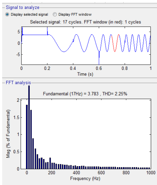
Fig 17 THD of the fuzzy controller based proposed system
