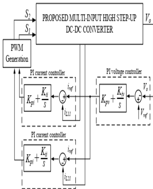
Figure 3. Control scheme of proposed multi-input high step-up dc-dc converter.
