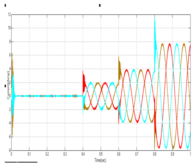
(b) PMSM Iabc Stator current
