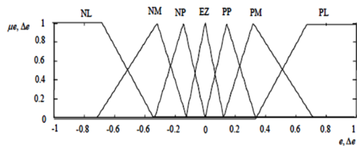
Fig.10. Input V_{dc} normalized membership function;
