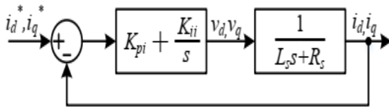
Figure 7. Block diagram of the PI current controller for the PMSM.
