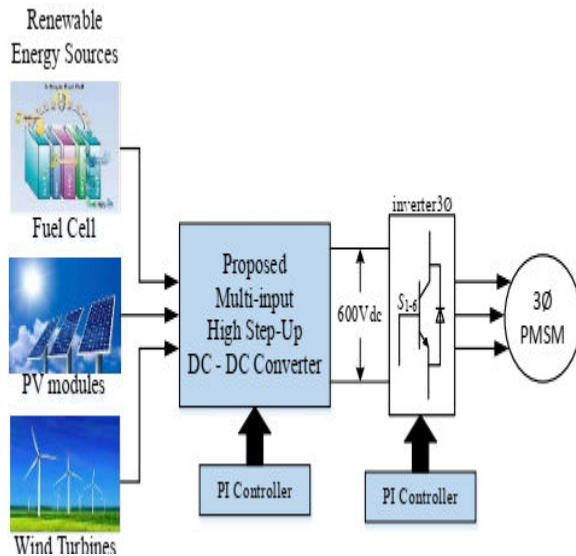
Figure 1. Overview structure of the proposed multi-input high step-up DC-DC converter for renewable energy-PMSM drive system.
