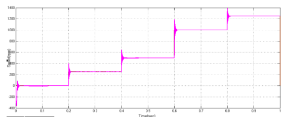
(c) PMSM Speed
