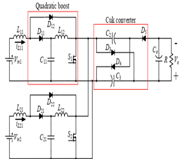
Figure 2. The proposed multi-input high step-up dc-dc converter.
