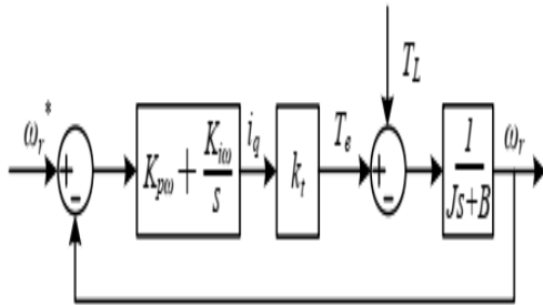
Figure 6. Block diagram of the PI speed controller for the PMSM.
