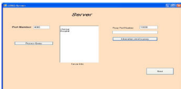
Fig.8 Server UI
