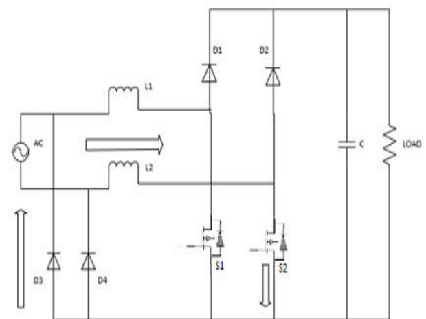
Fig.6. Mode III negative half cycle
