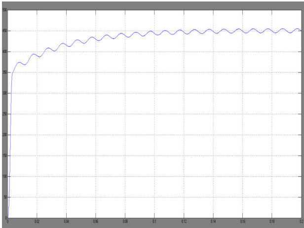
Fig.10 The output voltage regulation of Bridge Boost PFC Converter.
