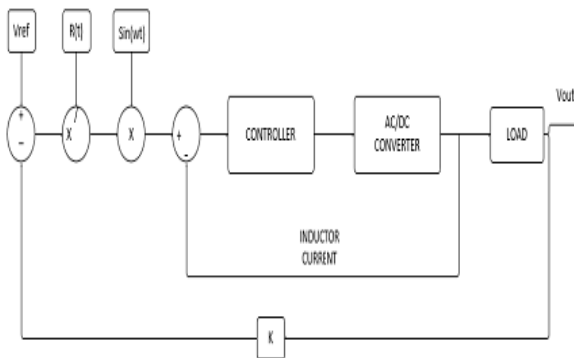
Fig.1. Block diagram of the control methodology of Boost PFC converter
