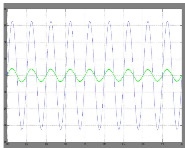
Fig.9. Current waveform and scaled voltage waveform of Bridge Boost Power Factor Correction Converter.
