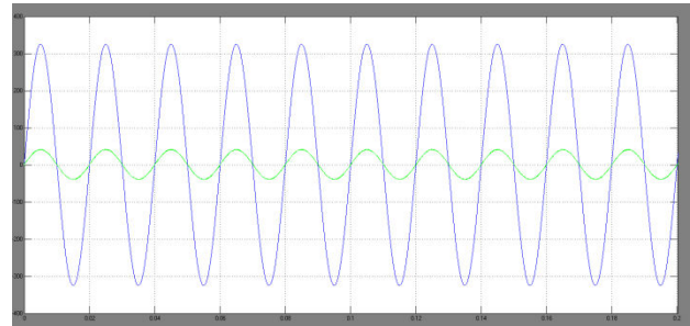
Fig.13. Current waveform and scaled voltage waveform of Bridgeless Boost Power Factor Correction Converter.
