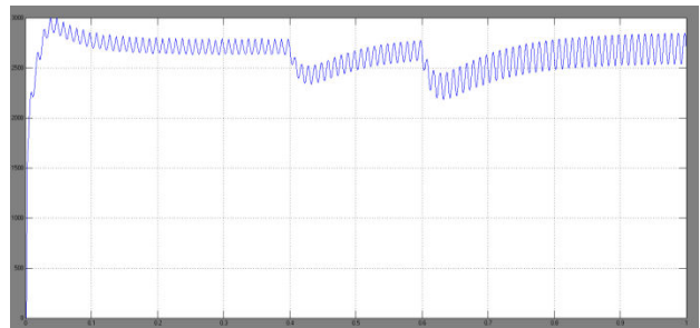
Fig.15. Output Power of the Bridgeless Boost PFC converter for switching loads of 1.28KW, 1.6KW & 2.13KW
