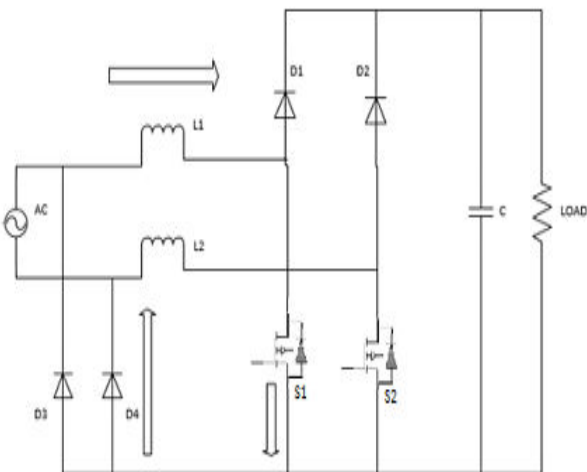
Fig.4. Mode I positive half cycle
