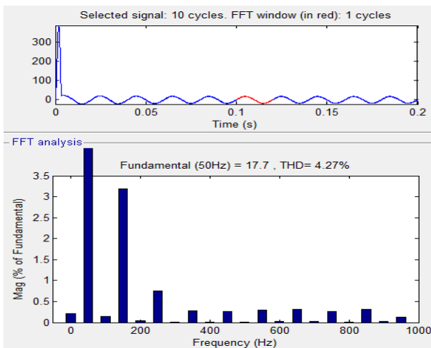
Fig.11. Frequency Response of input line current of Bridge Boost PFC Converter
