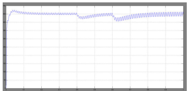
Fig.16. Output voltage regulation of the Bridgeless Boost PFC converter for switching loads of 1.28KW, 1.6KW & 2.13KW
