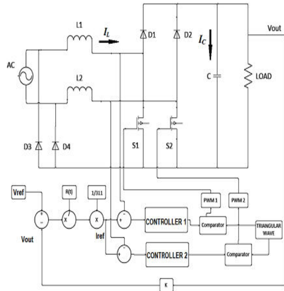
Fig.3. Schematic diagram of Bridgeless Boost PFC converter
