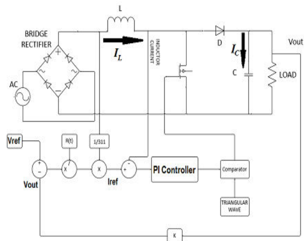
Fig.2. Schematic diagram of Boost PFC converter with control diagram
