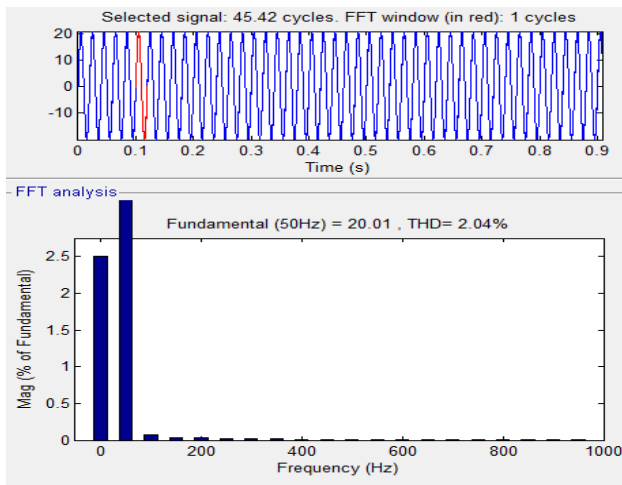
Fig.17. Frequency Response of input line current of Bridgeless Boost PFC Converter
