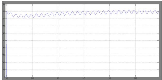
Fig.14. The output voltage regulation of Bridgeless Boost PFC Converter.
