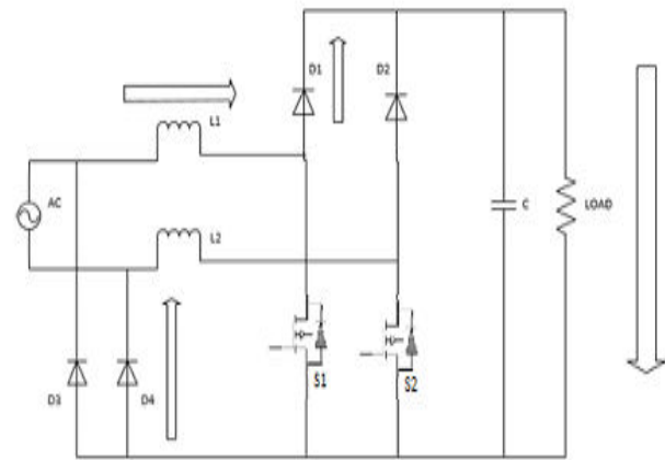
Fig.5. Mode II positive half cycle
