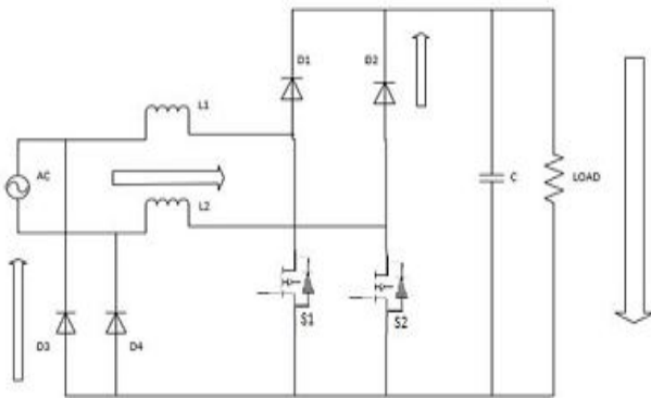
Fig.7. Mode IV positive half cycle V. INDUCTION MOTOR
