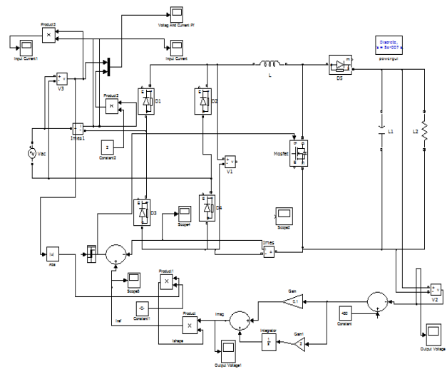
Fig.8 Matlab/Simulink model of bridge boost converter
