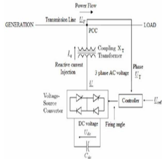
Fig 4: basic block diagram for static compensator.
