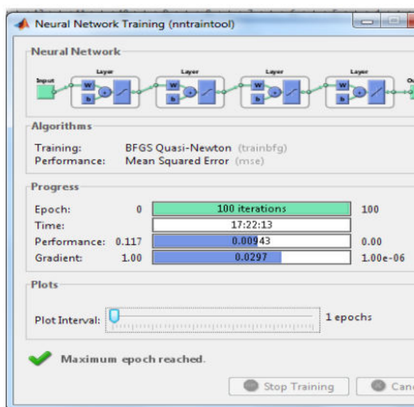
Fig. 4. TDNN Architecture
