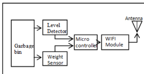
Fig. 1 Transmitter
