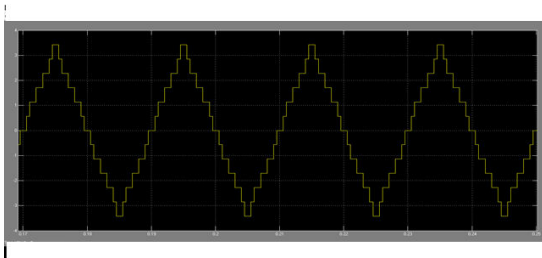
Fig. Output voltage levels of 13-level inverter
