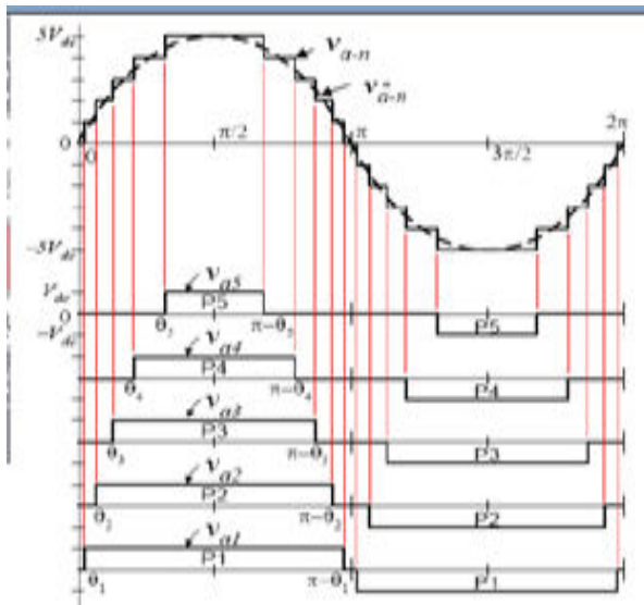
This figure shows the Output phase voltage waveform of an 11-level cascade inverter with 5 separate dc sources.
