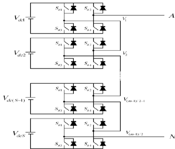
Figure shows Single-phase structure of a m level multilevel cascaded H bridge inverter.
