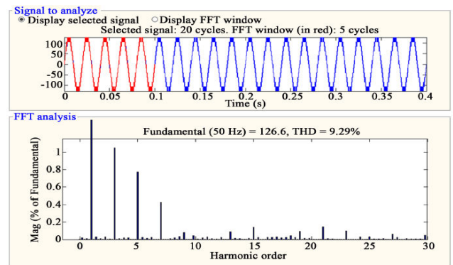
Fig 6: FFT analysis for 13-level inverter with R load.
