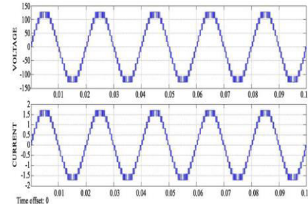
Fig 5: Output voltage and current waveform.
