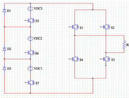
Fig 3: Proposed circuit for Cascaded 13-level Inverter-Asymmetric
