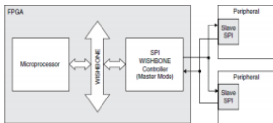
Fig 2 : Processor-SPI Interaction
