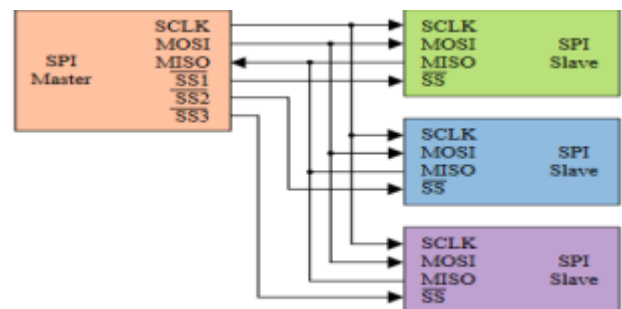
Fig 1 : SPI block diagram
