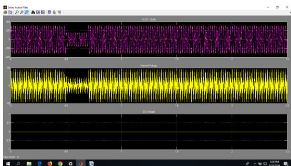
Fig.4.3. Voltage disturbances.
