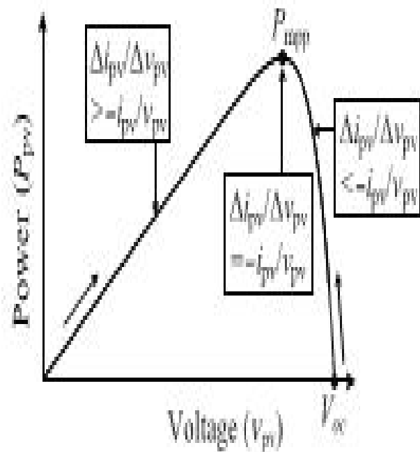
Fig.3. Illustration of INC-MPPT with SPV array P_{pv}-v_{pv} characteristics.
