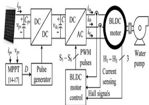
Fig.1. Conventional SPV-fed BLDC motor-driven water pumping system
