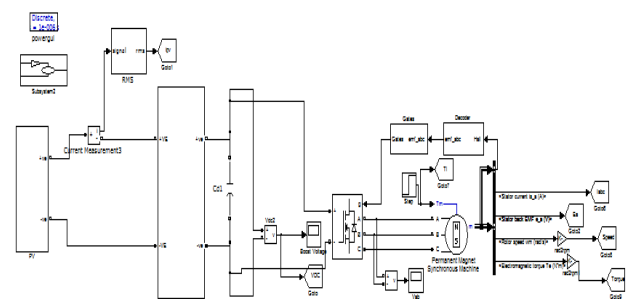
Fig. 4 Matlab/Simulink circuit of Starting and steady-state performances of the proposed SPV array-based zeta converter-fed BLDC motor drive for water pump
