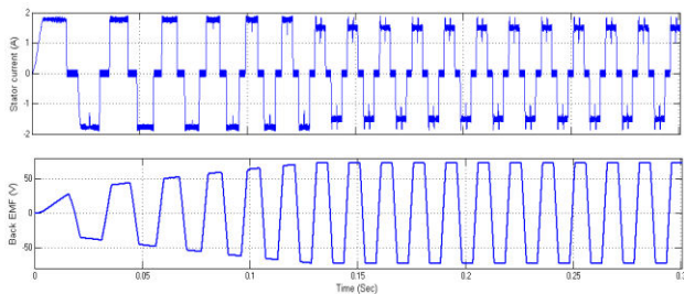
Fig.9 Stator current and emf.
