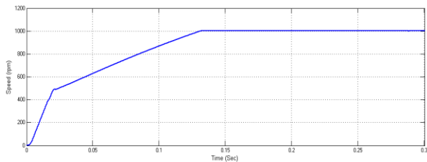
Fig.10 Speed.
