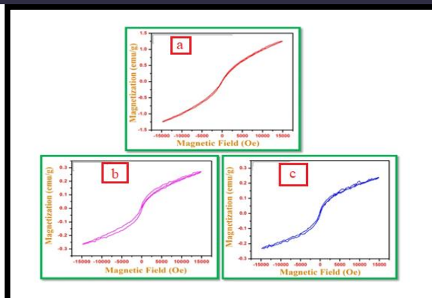
Figure.4 shows M-H curve of NiO nanoparticles (a)As-prepared, (b) 600^{\circ}\text{C} and (c) 800^{\circ}\text{C}
