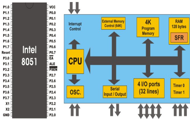
Figure 2.1: Architecture of 8052 Microcontroller
