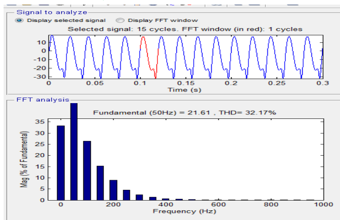
Fig 8 FFT analysis of source current waveform without STATCOM
