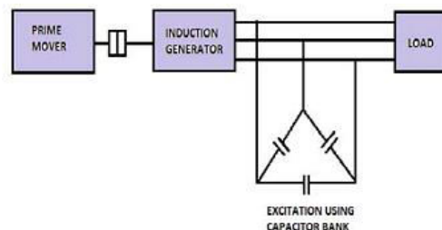
Fig 1.self excitation of induction generator
