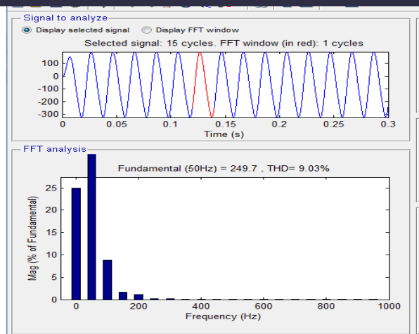
Fig 10 FFT analysis of source current waveform with STATCOM
