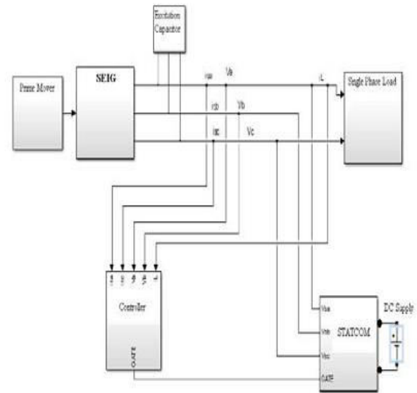
Fig 4 block diagram of SEIG-STATCOM model
