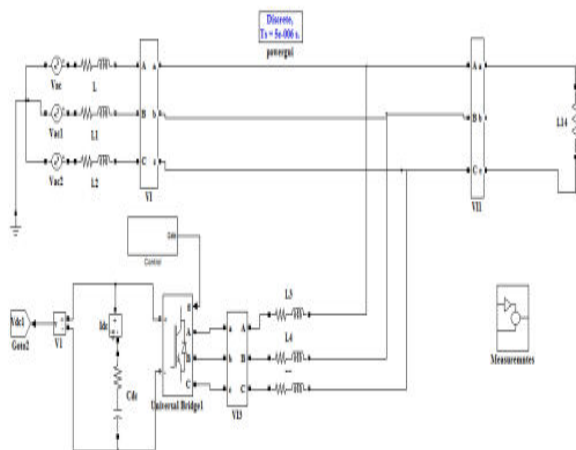
Fig 5 Matlab/simulation circuit of SEIG-STATCOM model
