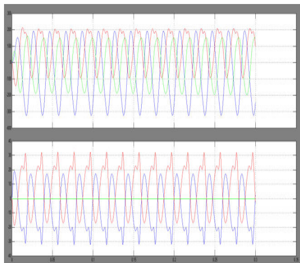
Fig 6 simulation wave form of voltage and current without statcom
