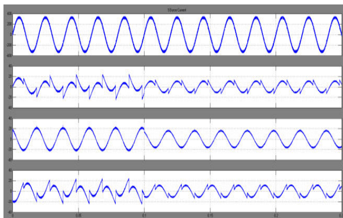
Fig 9 simulation wave form of wind SEIG source voltage, source current, compensation current and load current with single-phase loads.
