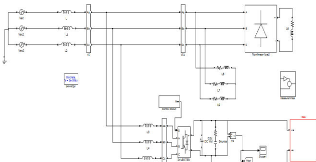
Fig.6 Matlab/Simulink of Proposed Statcom-Power Circuit
