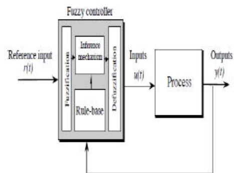
Fig.4. General Structure of the fuzzy logic controller on closed-loop system
