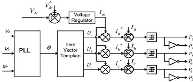
Fig. 2. Block diagram representation of grid-interfacing inverter control.
