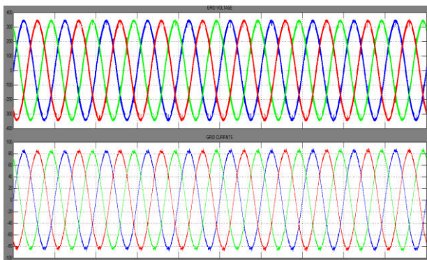
Fig.7 simulation results for grid side voltages and current
