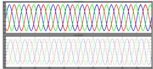
Fig.8 simulation results for load voltage and current
