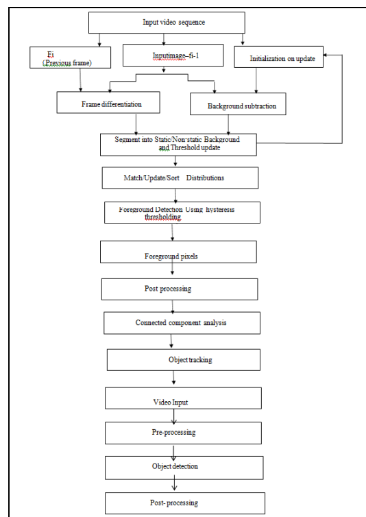
Fig 3. flow chart of object detection
