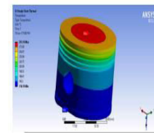
Fig 3.17: temperature of steel 8YSZ
