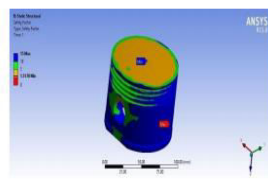
Fig 3.5: Safety factor of Al-alloy
