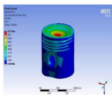
Fig 3.9: Stress of Lanthanum zirconate
