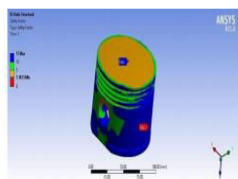
Fig 3.5: Safety factor of Steel
