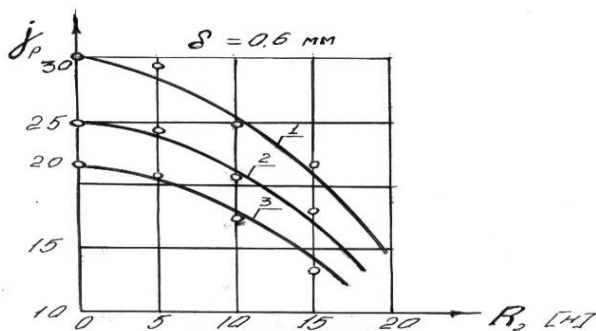
Fig. 5. Dependence of the operational rigidity of lamellar knife ( \delta=0.6 mm) from the value of R_2 . 1) N=400 H; 2) N=300 H; 3) N=200 H.
