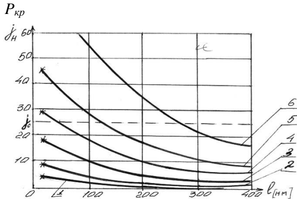
Fig. 4. Dependence of initial rigidity on the length of lamellar knife
