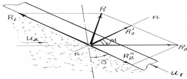
Fig. 1. Diagram of technological efforts arising during sliding cutting of food half-finished product with lamellar knife
