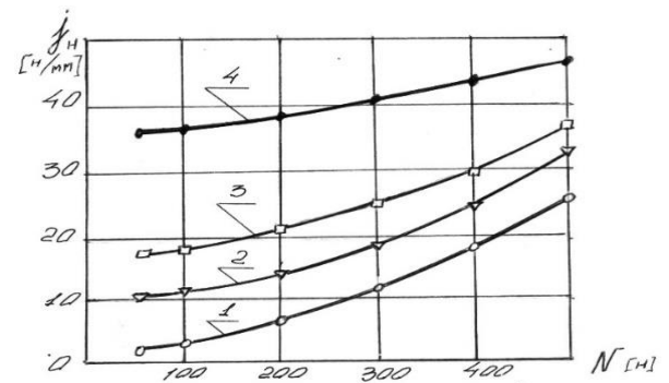
Fig. 3. Effect of tension on the initial rigidity of the lamellar knives 1- \delta = 0.2 mm; 2- \delta = 0.6 mm; 3- \delta = 0.8 mm; 4- \delta = 1.6 mm.
