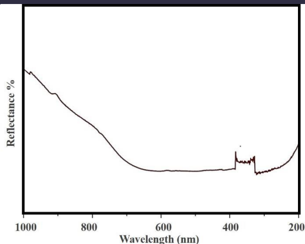
Fig. 2 DRS Pattern of PPy/ NiO nanocomposite
