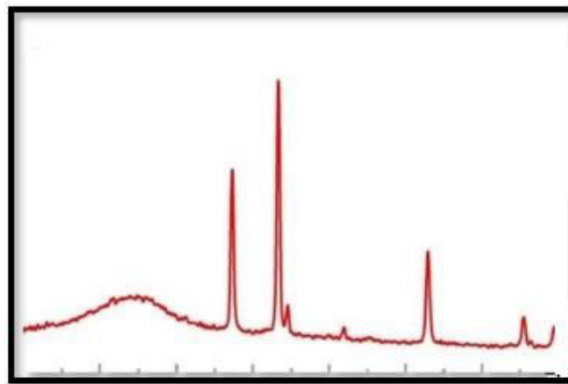
Fig. 1 XRD Pattern of PPy/ NiO nanocomposite
