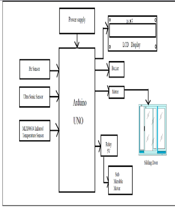
Fig.3 Block diagram of the project Sequence of the operation for door opening
