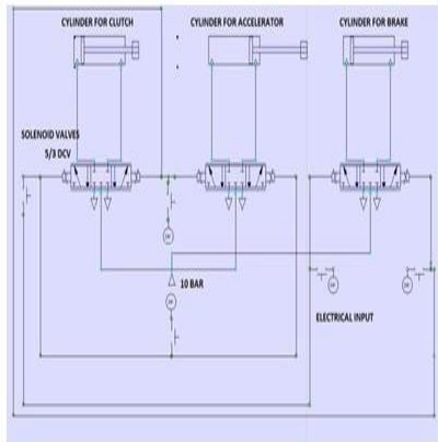
Figure 5: Pneumatic Circuit
