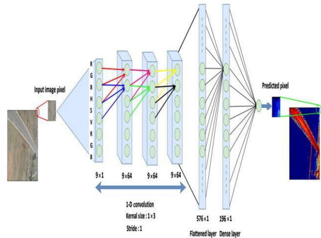
Figure 9: Architecture of end-to-end DNN, J-Net, used for autonomous driving
