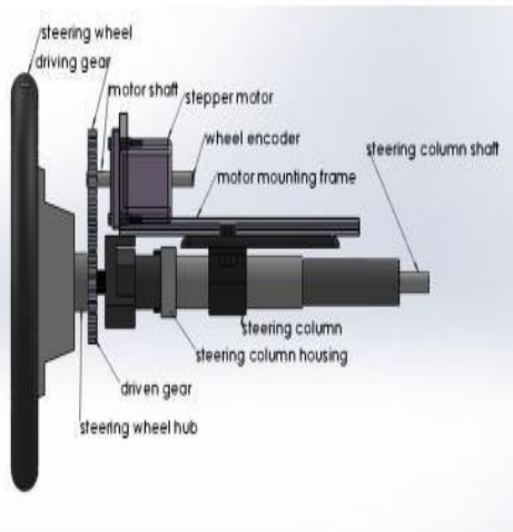
Figure 8: cad model
