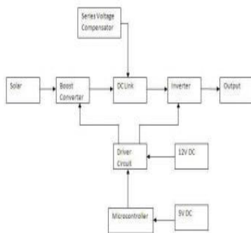
Fig.1 Block diagram of grid tie solar inverter by using series voltage compensator.
