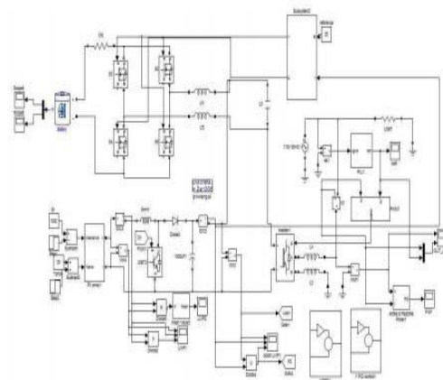
Fig-4- simulation circuit for grid tie solar inverter using series voltage compensator
