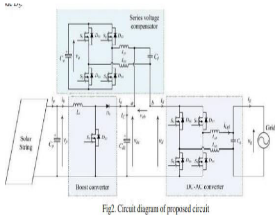
Fig2. Circuit diagram of proposed circuit
