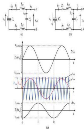
Fig 3. Ripple voltage on the input capacitor C_a in the compensator. (a) Operation when S_2 and S_3 are on. (b) Operation when S_1 and S_4 are on. (c) SPWM and the ripple voltage generated across C_a .
