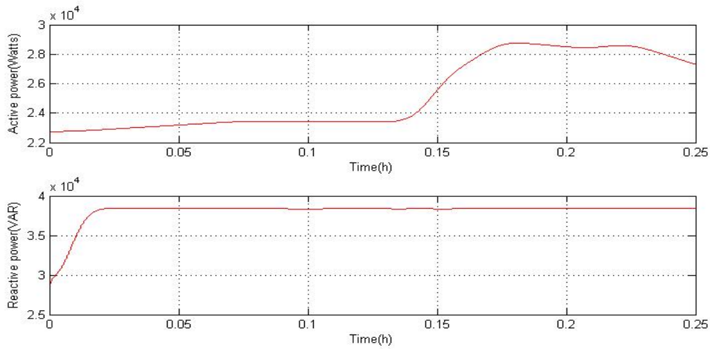
Figure 8: Simulation Result for Active and Reactive Powers at Load1 with ANN Controller
