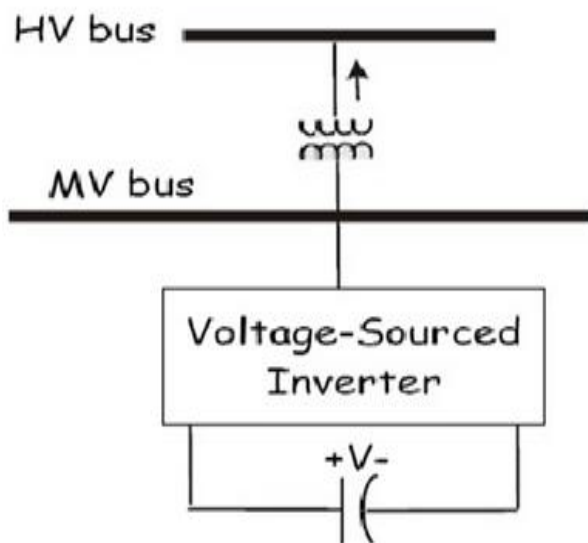
Figure 5: Operation of Converter
