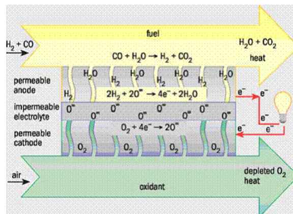
Fig 4: Operating principle of Fuel Cell
