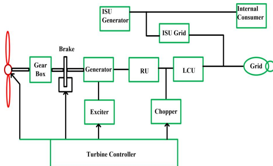
Fig. 3. Basic diagram of wind turbine
