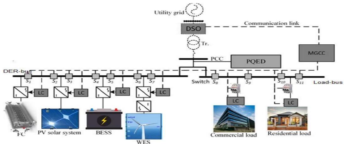
Figure 1: Diagram of an isolated MG with control system structure
