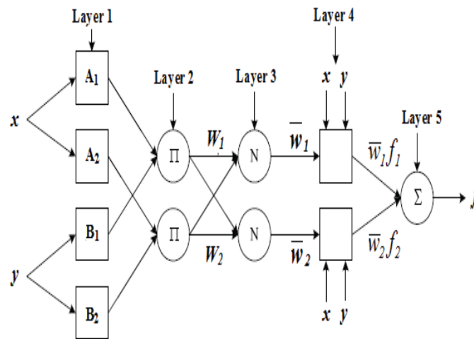
Fig 7 ANN architecture for a two-input multi-layer network
