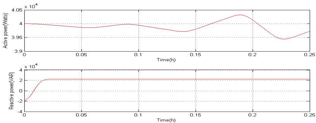
Figure 9: Simulation Result for Active and Reactive Powers at Load2 with ANN Controller
