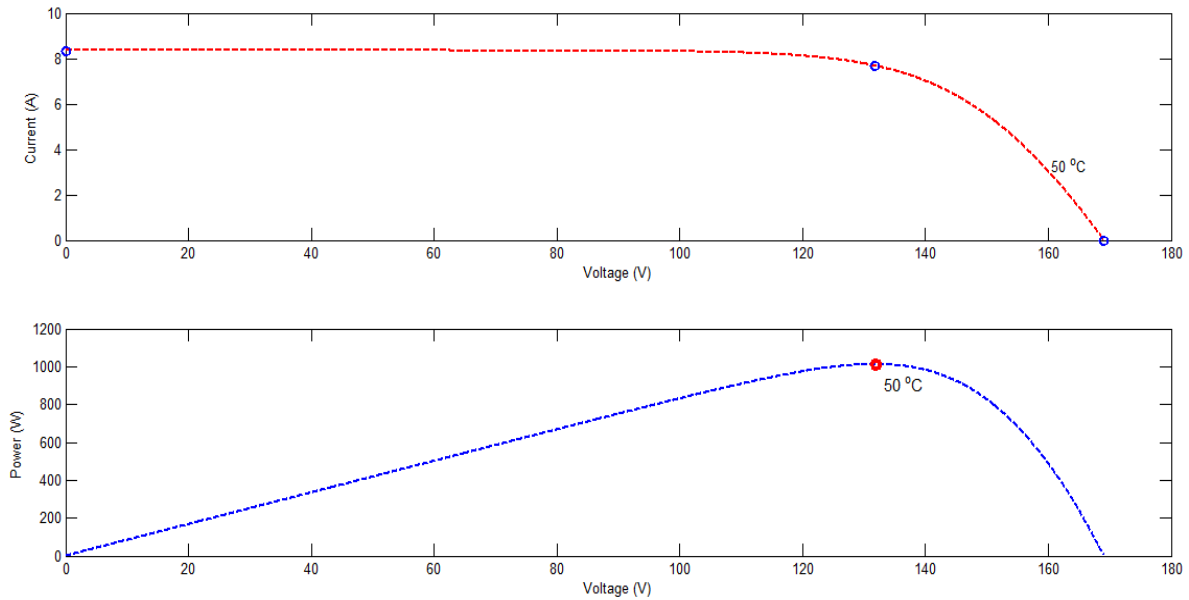
Fig. 2. Response of output characteristics of PV Array
