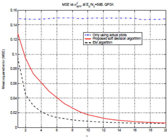
Figure 4: The MSE versus the variance of feedback information
