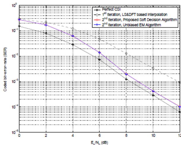
Figure 5: The BER performance of coded OFDM system
