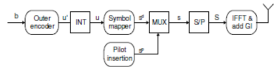
Figure 1: The transmitter structure of coded OFDM system
