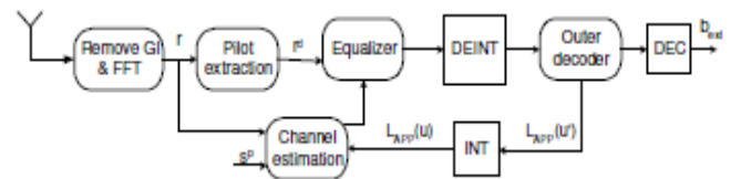
Figure 3: The receiver structure of coded OFDM system
