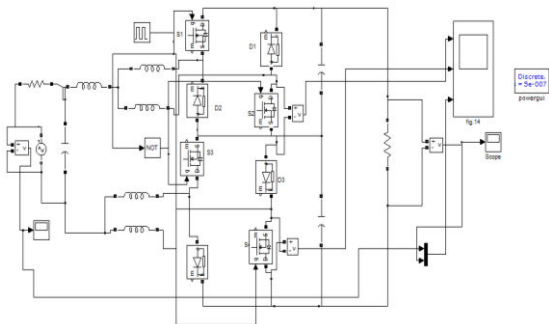
Fig.9 Simulink model of single-phase AC-AC converter
