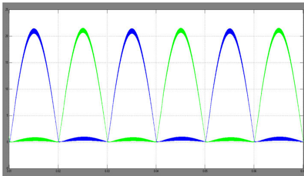
Fig.13. Experimental results with resistive load when D=0.4 . Current Wave forms of limiting inductors.
