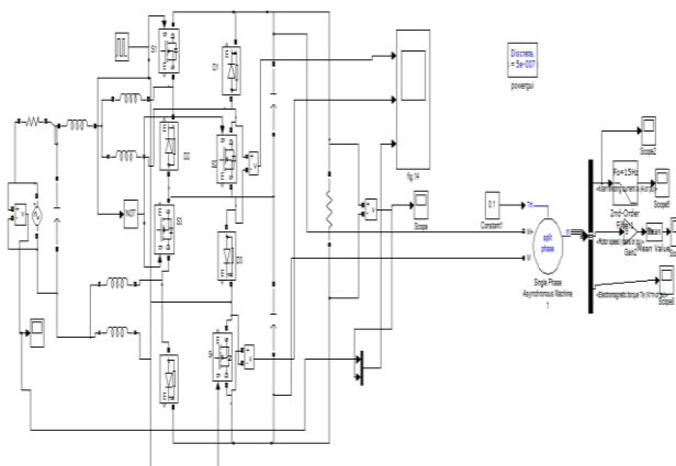
Fig.14 Simulink model of single-phase AC-AC converter with Induction Motor drive
