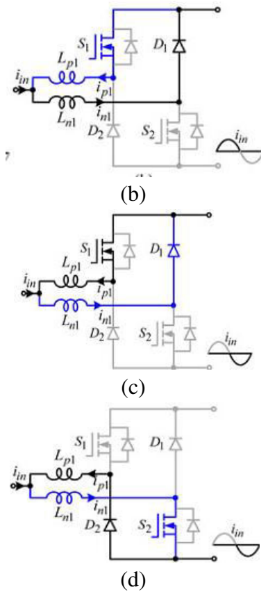
Fig.3. Conduction states of the proposed boost-type ac-ac converter. (a) i_{in} > 0 and S_2 on. (b) i_{in} > 0 and S_2 off. (c) i_{in} < 0 and S_1 on. (d) i_{in} < 0 and S_1 off.
