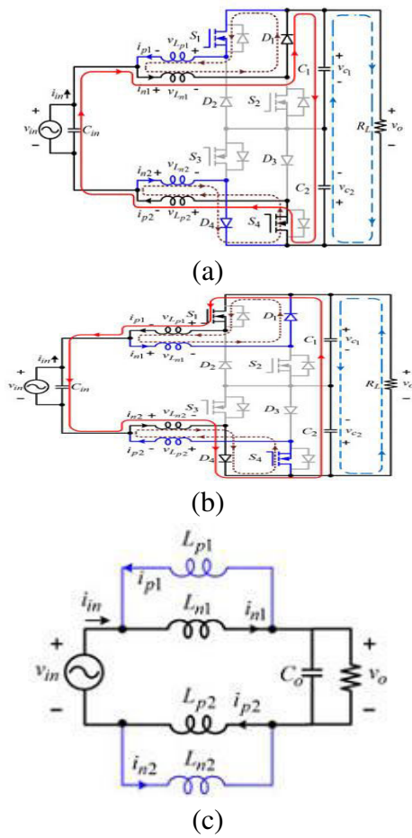
Fig.5. Mode 2 of the proposed boost type ac-ac converter.
