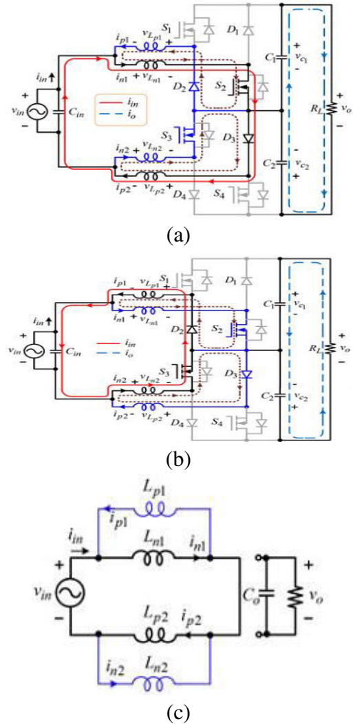
Fig.4. Mode 1 of the proposed boost-type ac-ac converter.
