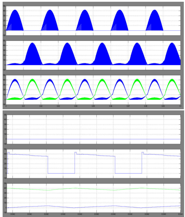
Fig.11 Experimental results with a resistive load when D=0.4 . (a) Waveforms of voltages across capacitors C1 and C2 and drain to source voltages of S2 and S4. (b) Magnification of waveforms in (a).
