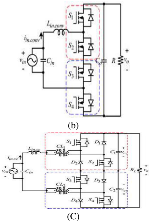
Fig. 1. Boost-type dc-dc and ac-ac direct PWM converters. (a) Traditional dc-dc converter. (b) Traditional ac-ac converter. (c) SC ac-ac converter [13]
