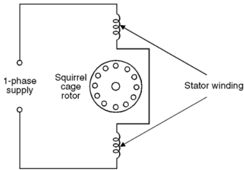
Fig.8 Single-phase induction motor
