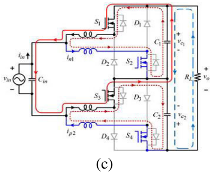
Fig.7. Operation of the proposed boost type ac-ac converter during overlap time. (a) Overlap time. (b) v_{in} > 0 . (c) v_{in} < 0 .
