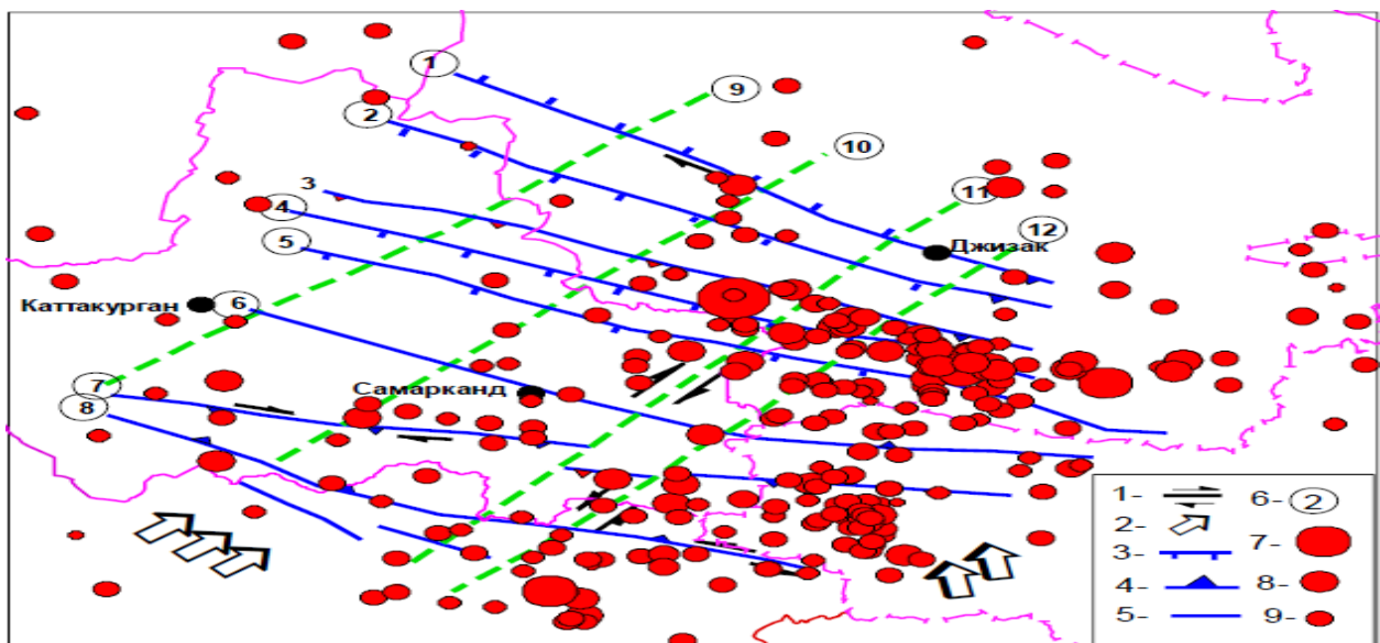
Figure 1. [1] Model of the latest tectonics of high-risk areas of Uzbekistan
