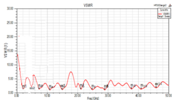
Fig 4: VSWR versus frequency of the antenna.
