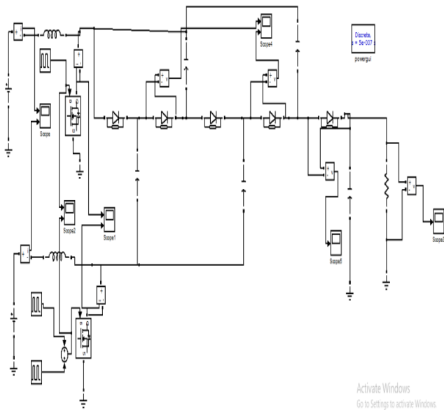
Fig 1: Simulation modeling of high-voltage-gain dc-dc converter
