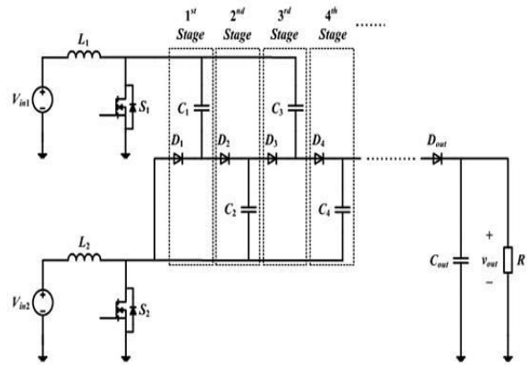
Fig.8. Alternative to the proposed converter with N number of VM stages
