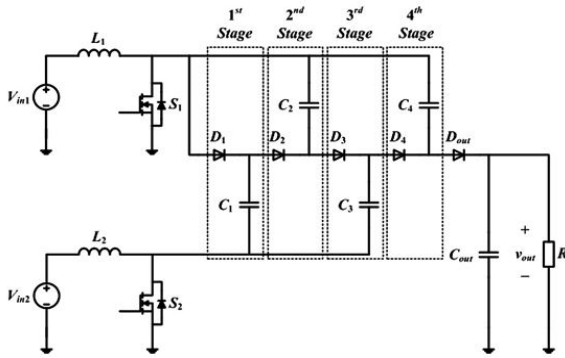
Fig.2. Proposed high-voltage-gain dc-dc converter with four VM stages
