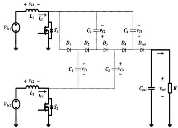
Fig.4. Mode-I of operation for the proposed converter with four VM stages
