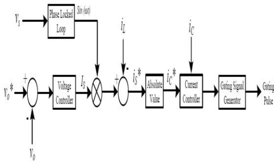
Fig 11 Adopted control scheme for the Closed Loop operation
