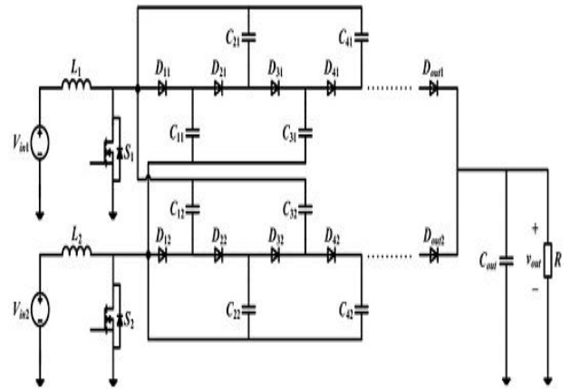
Fig.10. Combined topology with N number of VM stages
