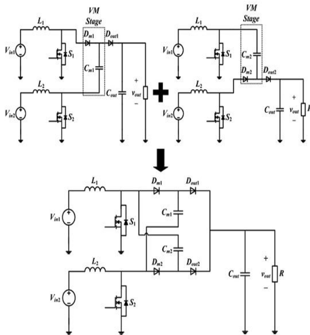
Fig.9. Combined topology with single VM stage
