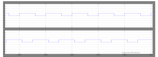
Fig 3: Simulation Waveforms of Inductor Currents at even stage
