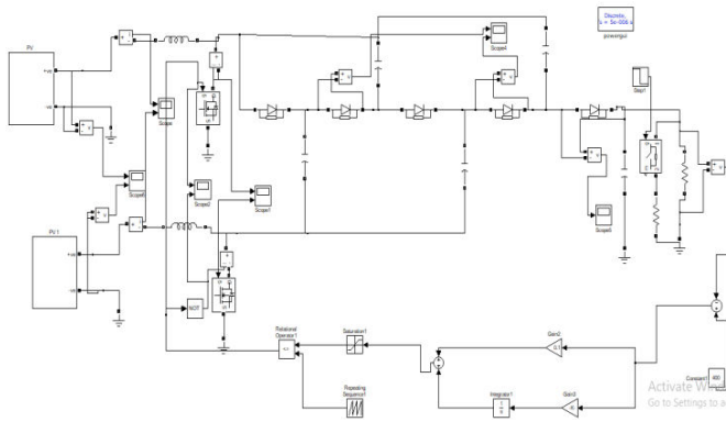
Fig 7: Simulation modeling of PV with Closed loop Circuit
