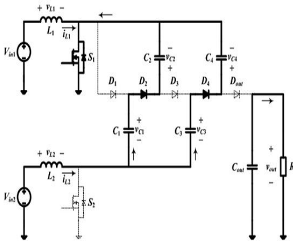
Fig.6. Mode-III of operation for the proposed converter with four VM stages
