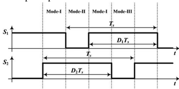
Fig.3. Switching signals for the input boost stage for the proposed converter
