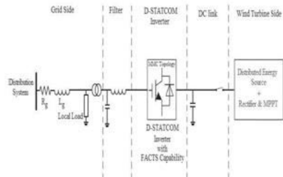
Fig. 1. Complete configuration of the proposed inverter with FACTS capability.
