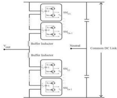
Fig.2. Structure of a single-phase MMC inverter structure.
