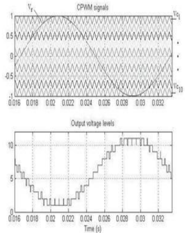
Fig. 4. CPWM waveforms for an 11-level MMC inverter, and the generated output voltage levels.
