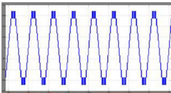
Fig. 8.Simulated output voltage of an 11-level inverter.
