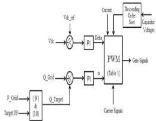
Fig. 3. Schematic of the proposed controller system.
