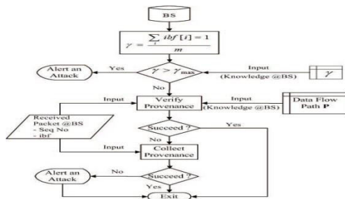
Fig.2: System Architecture
