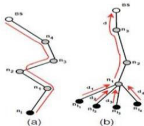
Fig.1: Provenance Graph
