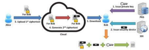
Fig. 1: Ordinary Data Sharing.
