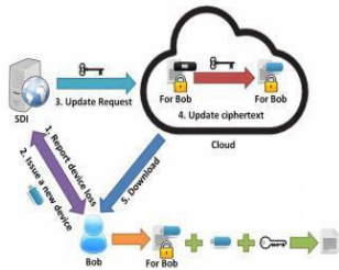
Fig. 2: Update Ciphertext after Issuing A New Security Device.
