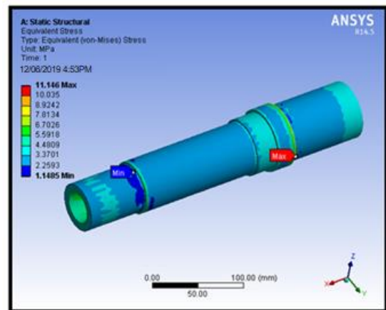
STRESS
