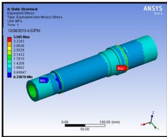
STRESS
