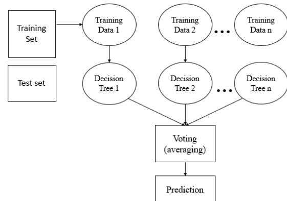
Fig. 2: Random Forest algorithm.
