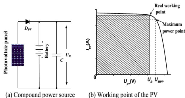
Fig.6 Power supply at mode 2
