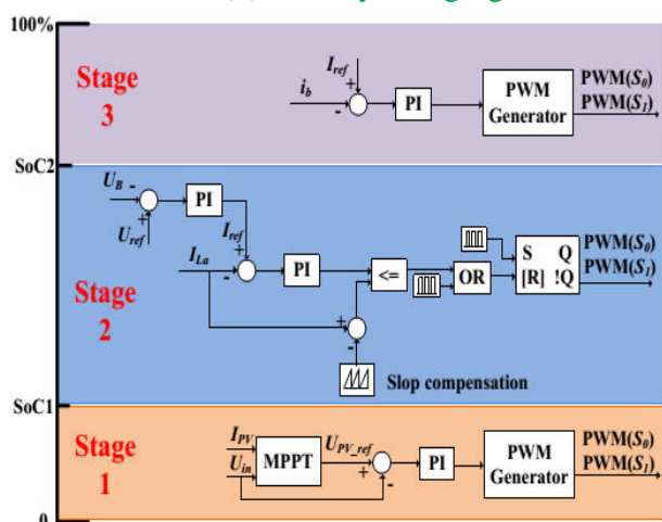
(c) Charging control strategy.
