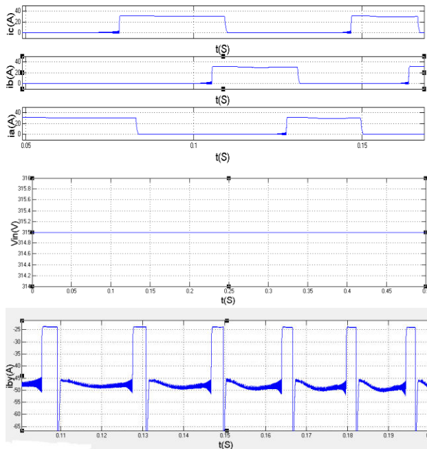
(a) Simulation results of driving-charging mode (mode 1)
