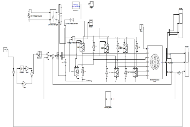
Fig.16 SRM drive model diagram
