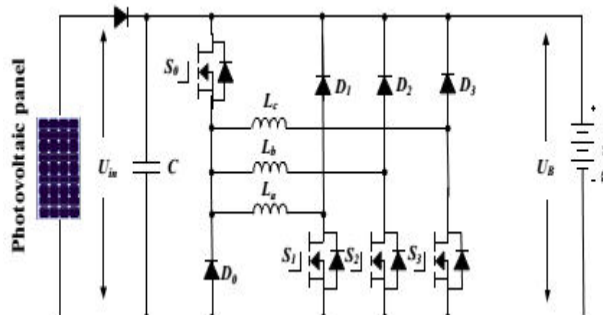
(b) Operation circuit under mode 2
