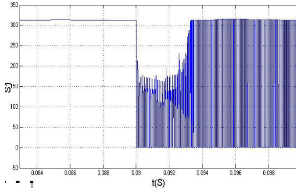
(a) Grid charging (mode 5)
