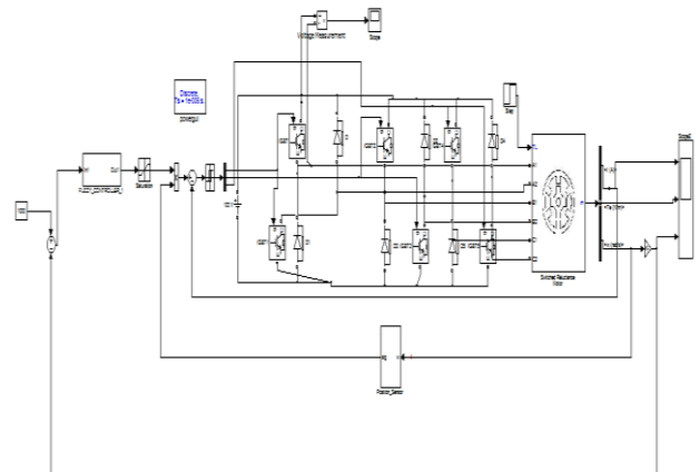
Fig.24 SRM drive model diagram With Fuzzy controller
