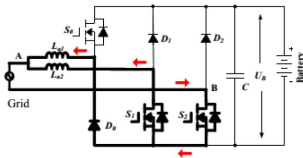
(c) Grid charging state 3 ( U_{grid} < 0 )
