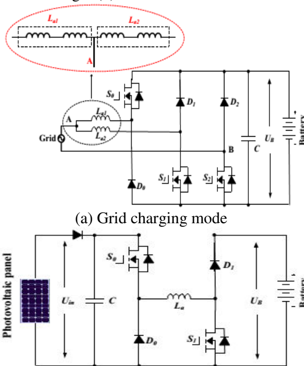
(a) Grid charging mode (b) PV source charging mode Fig.5 Equivalent circuits of charging condition modes
