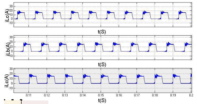
(b) Simulation results of single source driving mode (modes 3 and 4)
