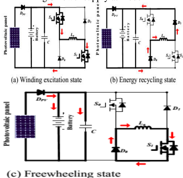
Fig.7 Working states at mode 2
