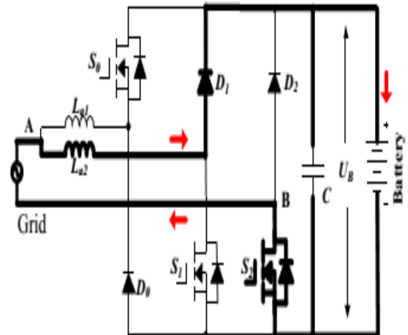
(b) Grid charging state 2 ( U_{grid} > 0 )
