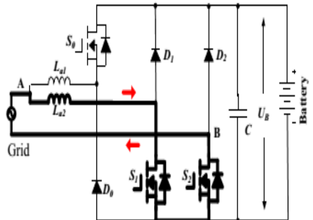
(a) Grid charging state 1 ( U_{grid} > 0 )
