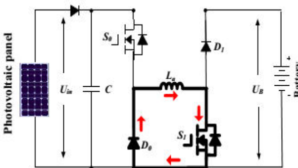
(c) Freewheeling state
