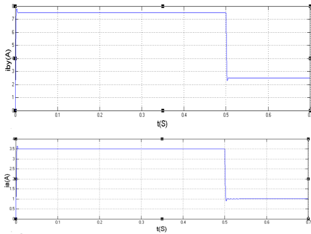
(c) PV charging mode 6 (stage 2 to stage 3) Fig.21 simulation results for charging modes.
