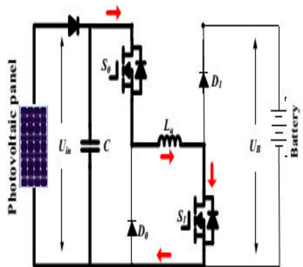
(a) Phase inductance charging
