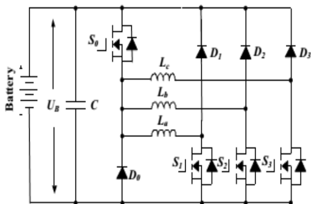
(d) Operation circuit under mode 4 Fig.4 The equivalent circuits under driving modes
