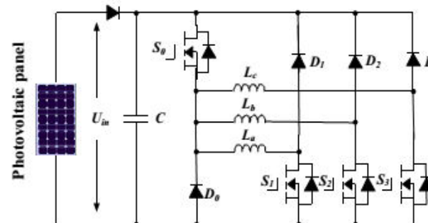
(c) Operation circuit under mode 3
