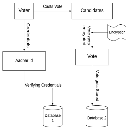
Figure 3.1. Process of voting using Blockchain
