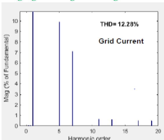
Fig.7. The harmonic spectrum of grid current
