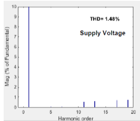
Fig 8. The harmonic spectrum of supply voltage
