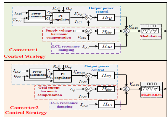
Fig. 3. Diagram of the proposed interfacing converter control strategies.
