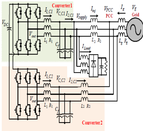
Fig. 2. Diagram of the proposed topology.
