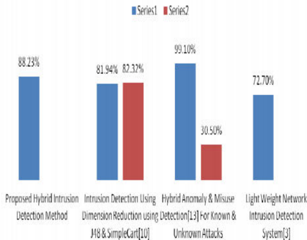
Figure 3. Comparative Analysis In Terms of Detection Accuracy
