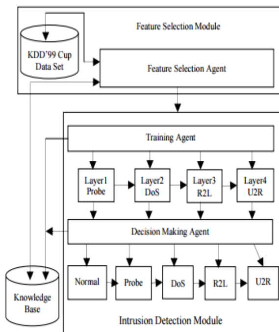
Figure 1. System Architecture
