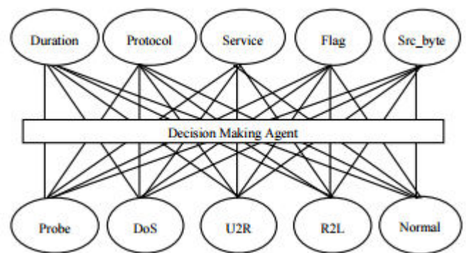
Figure 2. Graphical representation of CRF
