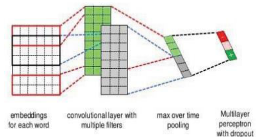
Figure 1: Diagram representing a convolutional neural network
