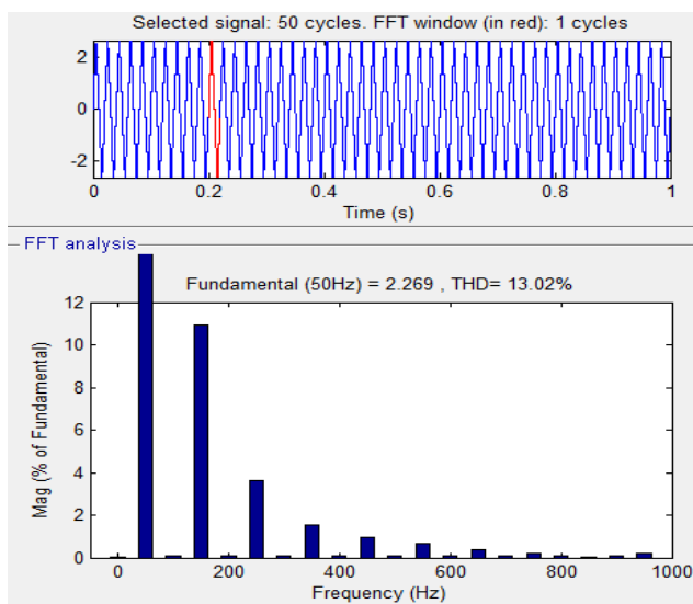
Fig.15. Simulation waveform of R Load THD
