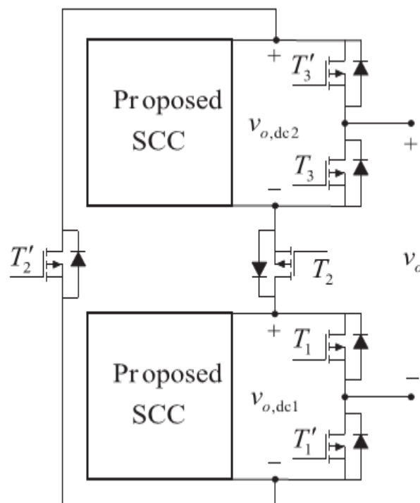
Fig.3. Proposed SMLI configuration.
