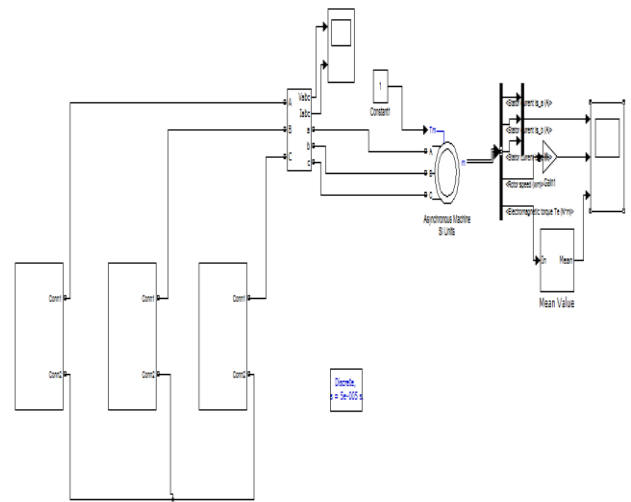
Fig.20.Matlab circuit for proposed SMLI configuration with R Load
