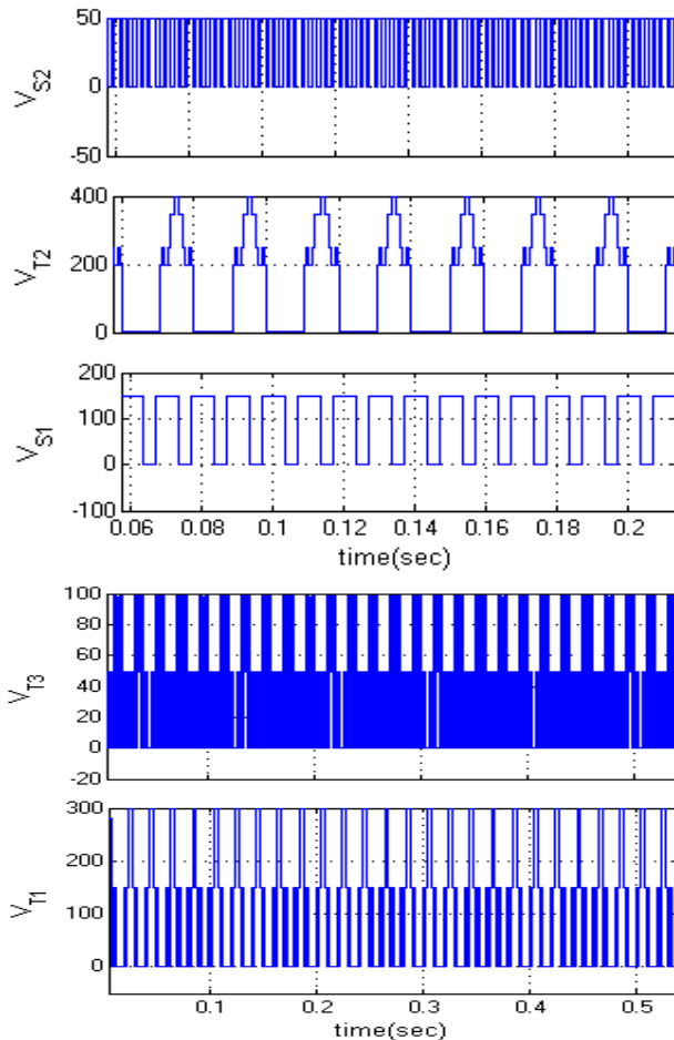
Fig.14. Simulation Voltage waveforms across switches at R Load
