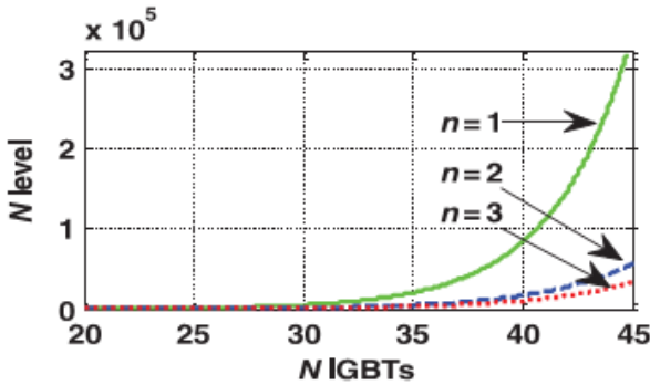
Fig.5. Variation of N_{level} against N_{IGBT} for different values of n .
