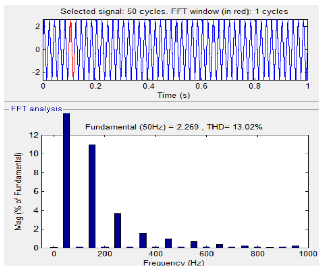
Fig.19.Simulation waveform of THD at RL LOAD
