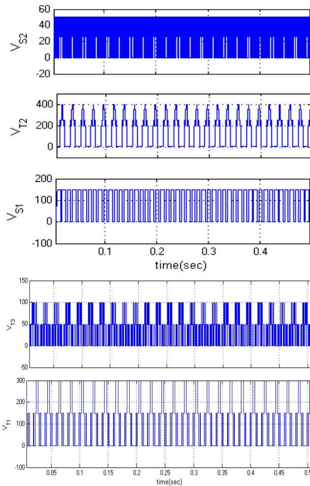
Fig.18.Simulation waveform of Switch voltages of RL Load
