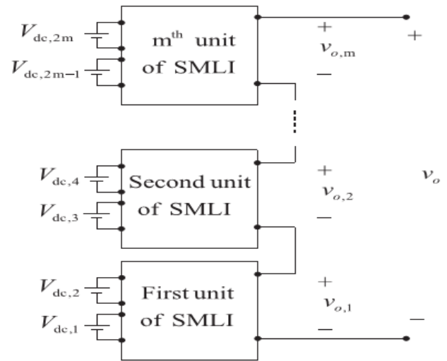
Fig.4. Proposed CSMLI
