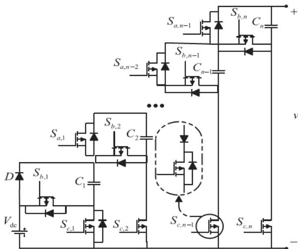
Fig.2. Proposed SCC
