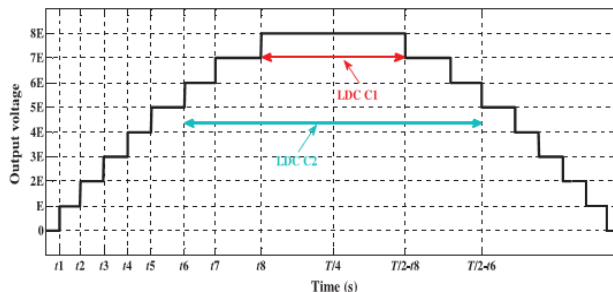
Fig.7. Typical output voltage waveform of 17-level inverter for positive half-cycle.
