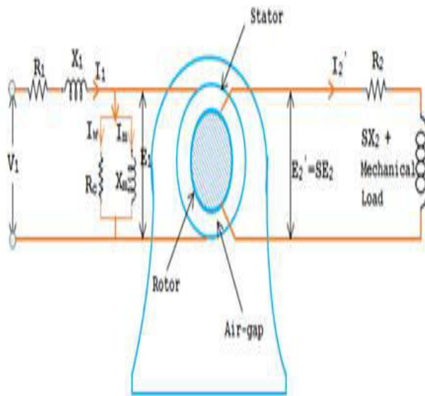
Fig.10. Equivalent circuit for Induction motor
