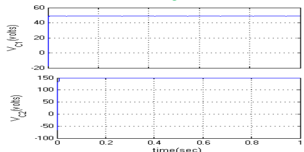
Fig.13. Simulation waveforms for Capacitors' voltage ripple waveforms R Load
