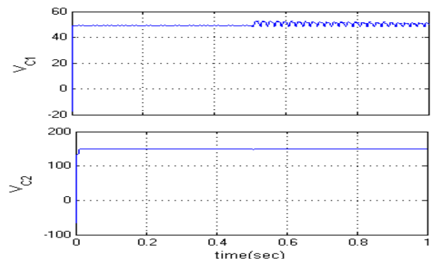
Fig.17. Simulation waveforms for Capacitors' voltage ripple waveforms RL Load
