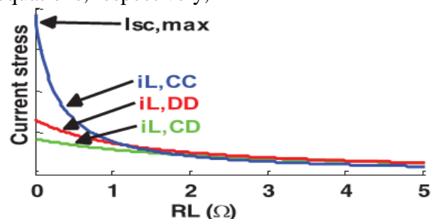
Fig.9. Variation of current stresses versus R_L in three defined modes
