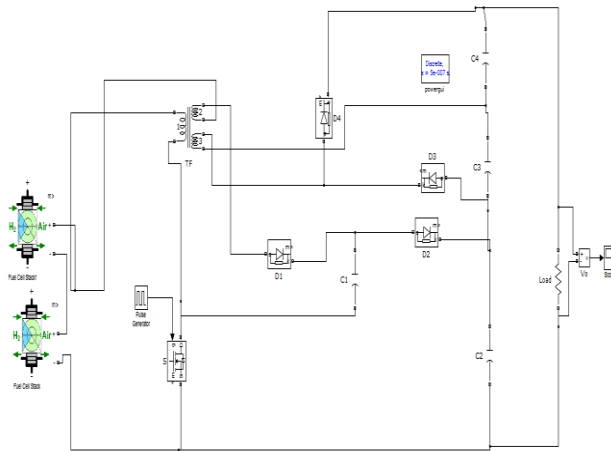
Fig. 13. Matlab/Simulation model of high step up Converter with fuel cell.
