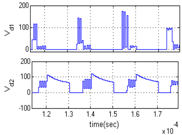
Fig.10.Simulation waveform of diode Voltage ( V_{d1} ), diode Voltage ( V_{d2} ).
