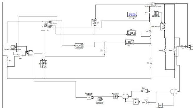
Fig.19.Matlab/simulation model of Closed loop Control of high step up Converter with Decremental load.
