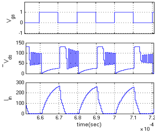
Fig.7.Simulation waveform of gate voltage ( V_{gs} ), diode Voltage ( V_{ds} ), Input Current ( i_{in} ).
