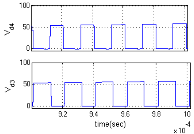
Fig.11.Simulation waveform of diode Voltage ( V_{d4} ), diode Voltage ( V_{d3} ).
