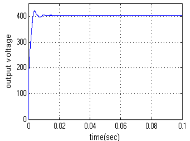
Fig.12.output Voltage of high step up Converter.
