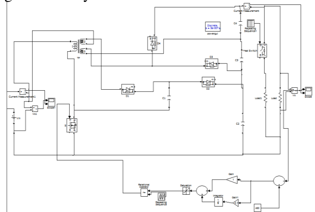
Fig. 17. Matlab/simulation model of Closed loop Control of high step up Converter with Incremental load.
