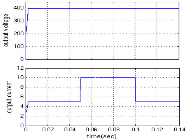
Fig.18.output voltage & current of closed loop High step up converter with Incremental load.
