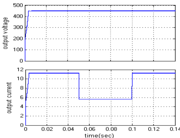
Fig.20.output voltage & current of closed loop High step up converter with Decremental load.
