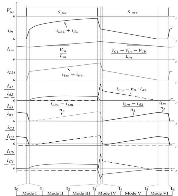
Fig. 3. Steady-state waveforms in CCM operation.
