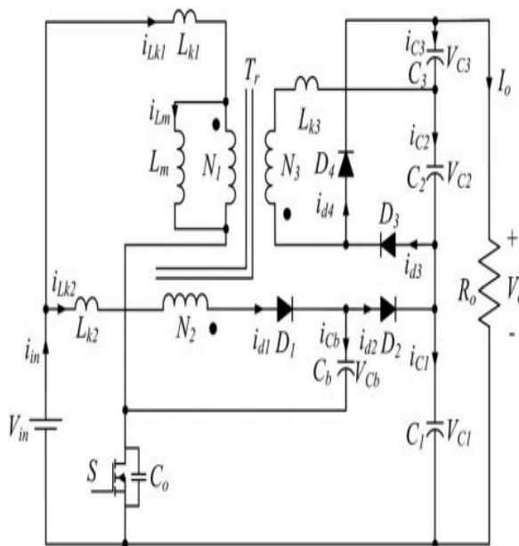
Fig. 2. Equivalent circuit of the proposed converter.
