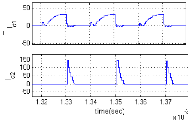
Fig.8.Simulation waveform of diode Current ( I_{d1} ), diode Current ( I_{d2} ).
