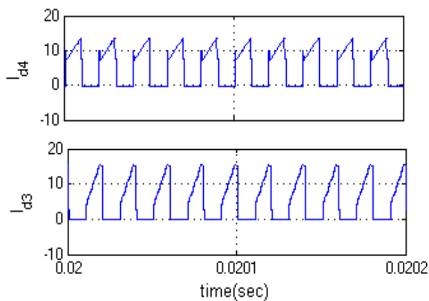
Fig.9.Simulation waveform of diode Current ( I_{d4} ), diode Current ( I_{d3} ).
