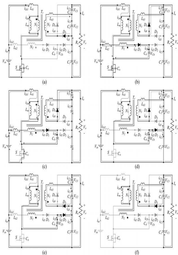
Fig. 4. CCM operating modes of the proposed converter. (a) Mode I [t0, t1]. (b) Mode II [t1, t2]. (c) Mode III [t2, t3]. (d) Mode IV [t3, t4]. (e) Mode V [t4, t5]. (f) Mode VI [t5, t6].
