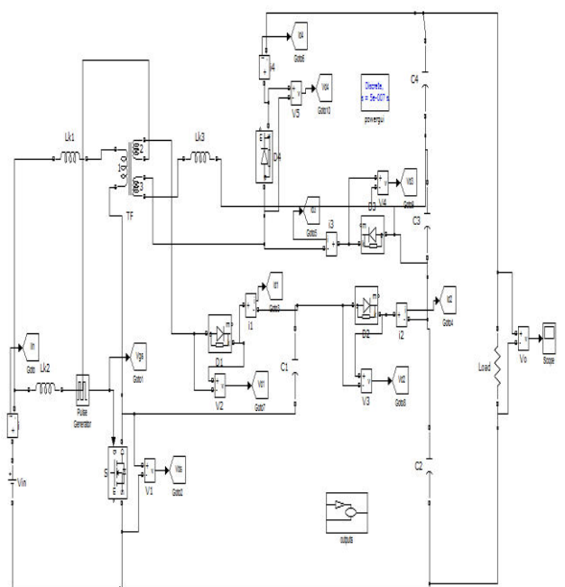
Fig.6. Matlab/simulation model of high step up Converter.
