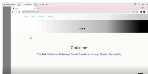
Fig.8: Prediction result
