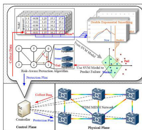
Fig.2: System architecture
