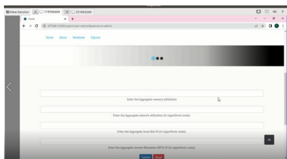
Fig.6: Main screen
