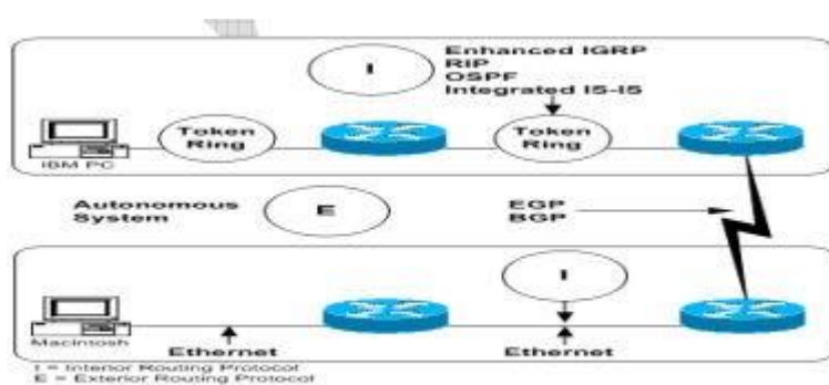
Fig. 3: Routing methods
