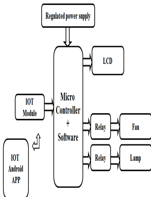
Fig. 1: Block Diagram using Microcontroller.
